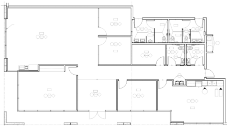
OFFICE PLAN | 2,949 SF
